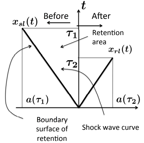
FIGURE 8. Retention after stopping production process
