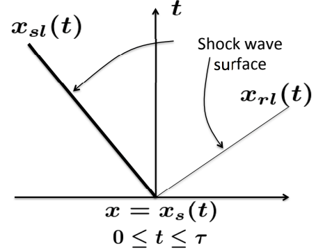
FIGURE 10. Bottle neck point x = x_s(t)
