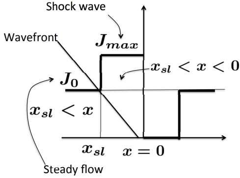
FIGURE 5. Shock wave generation due to suspension of production at x = 0
