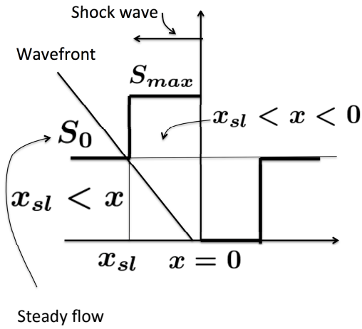
FIGURE 7. Shock wave generation due to suspension of production at x = 0
