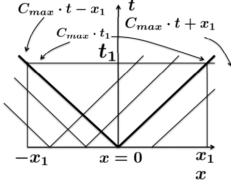
FIGURE 11. Characteristic curve of shock wave
